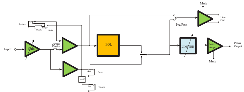
Block Diagram - AG1000
